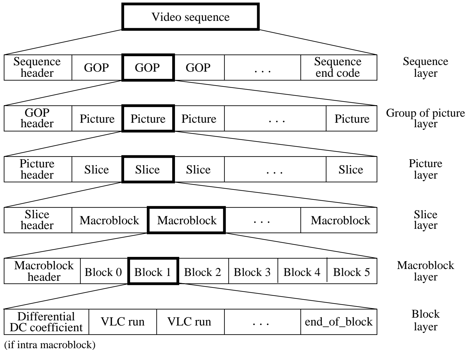
Fig 11.5: Layers of MPEG-1 Video Bitstream.
