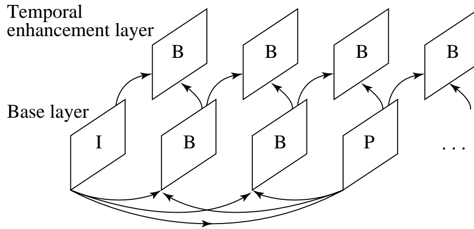
(b) Interlayer Motion-Compensated (MC) Prediction.
