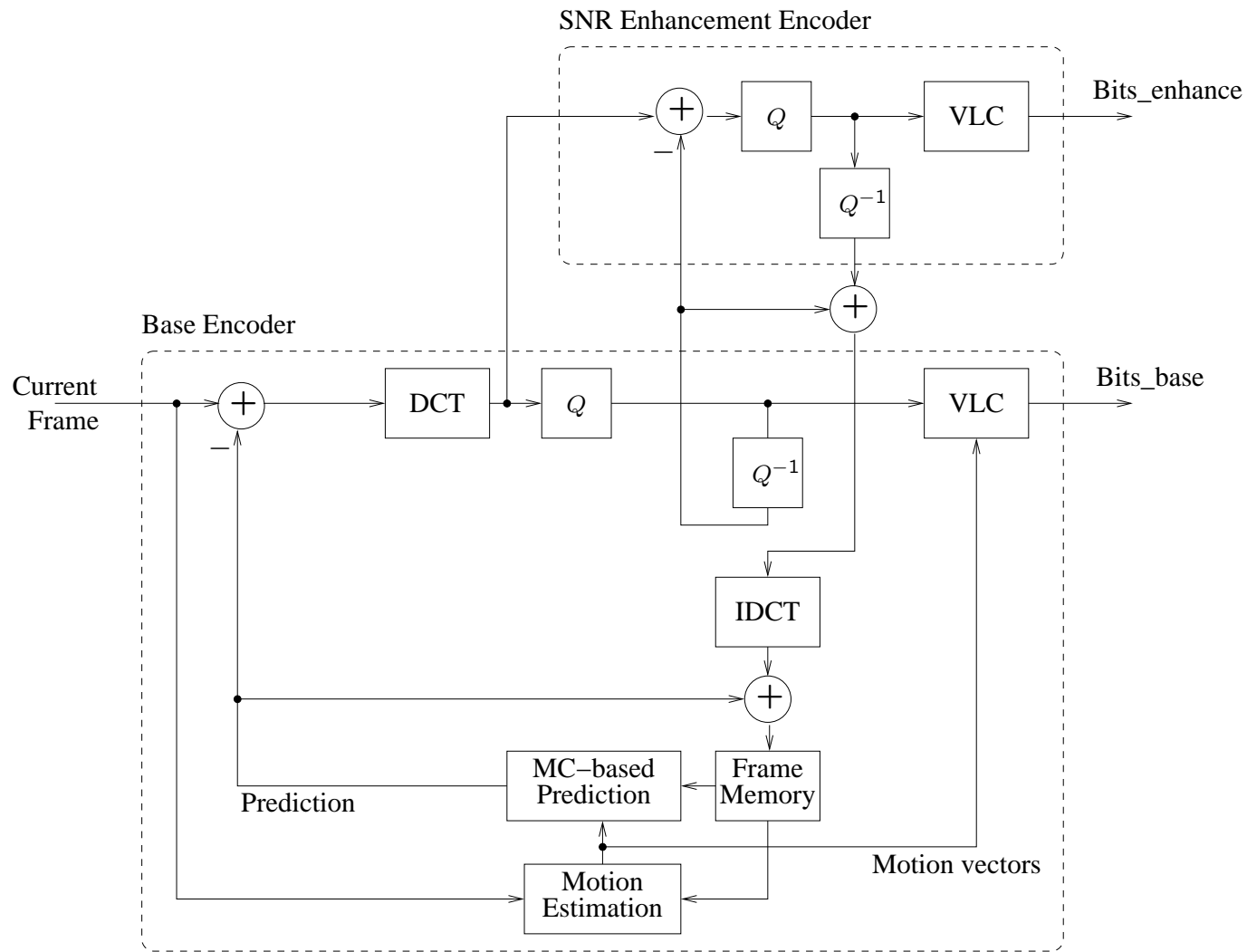
(a) Encoder
